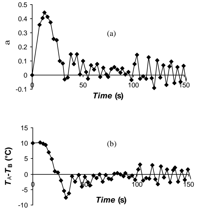
Fig. 3. Results of ex-vivo experiment #2, 12 min ablation with two probes. The time course of (a) control variable \mathbf{a} , and (b) difference in average tip temperature between probes A and B, is shown for first 150 s of the experiment.
